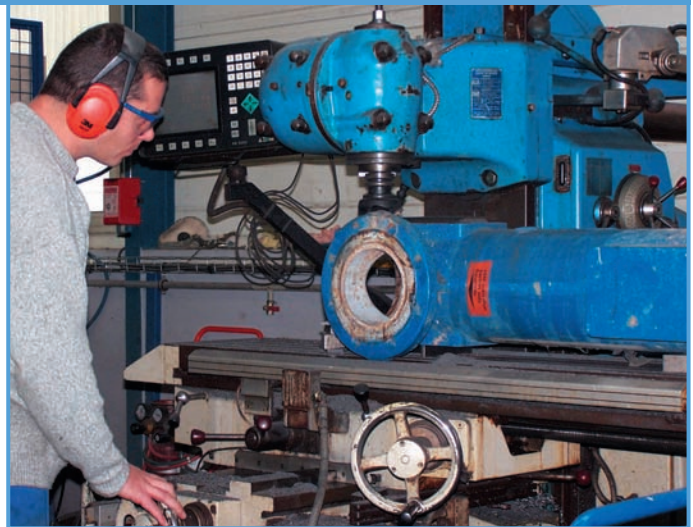
Overhaul of a pump with creation of inspection doors on the pump body
